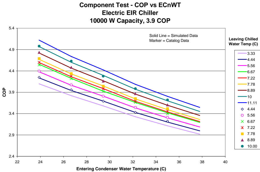
Figure 6 Chiller COP Versus Entering Condenser Water Temperature
