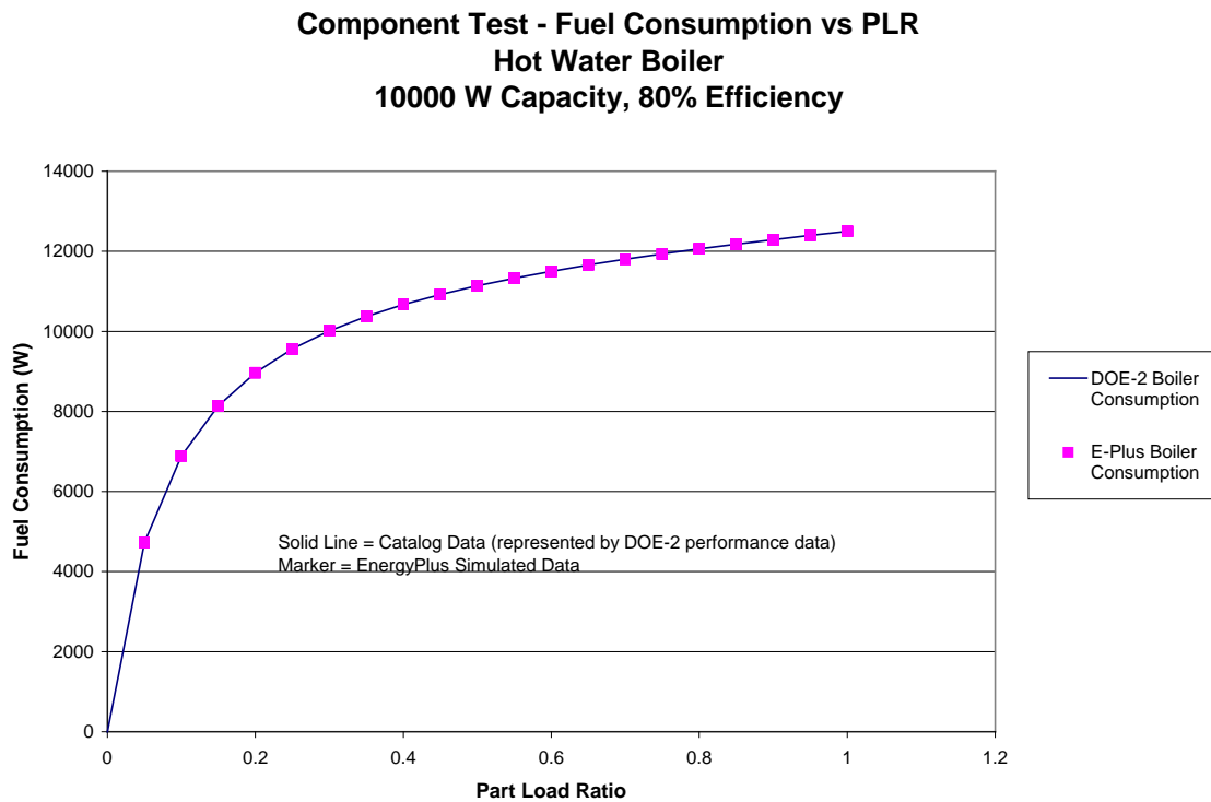
Figure 9 Hot Water Boiler Fuel Consumption Versus Part Load Ratio – EnergyPlus Model Versus DOE-2 Performance Curve
