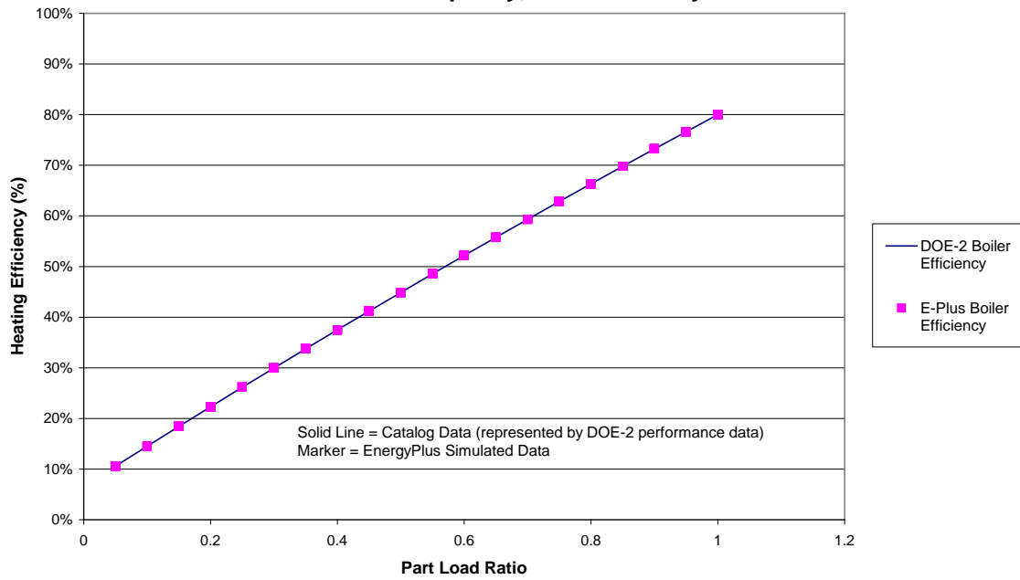
Figure 10 Hot Water Boiler Heating Efficiency Versus Part Load Ratio – EnergyPlus Model Versus DOE-2 Performance Curve
