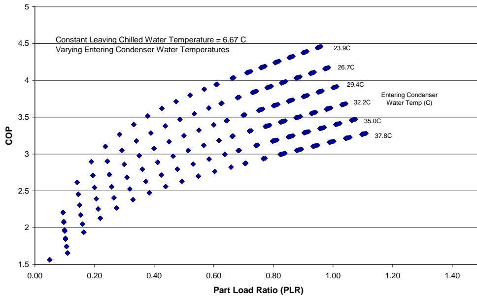
Figure 8 Chiller COP Versus Part Load Ratio
