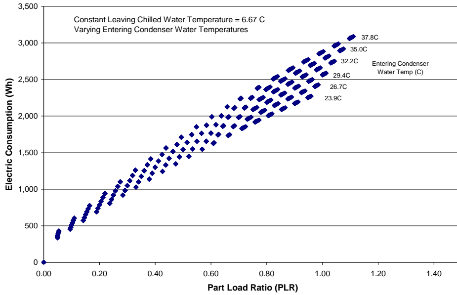
Figure 7 Chiller Electric Consumption Versus Part Load Ratio
