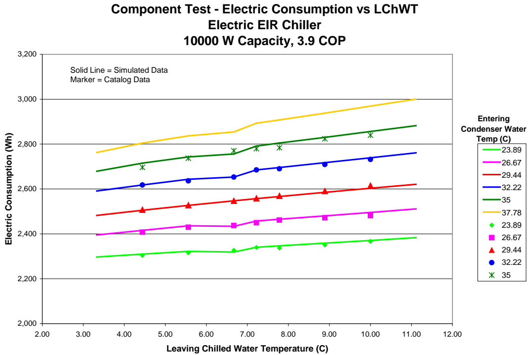
Figure 3 Chiller Electric Consumption Versus Leaving Chilled Water Temperature – EnergyPlus Model Versus Manufacturer Data
