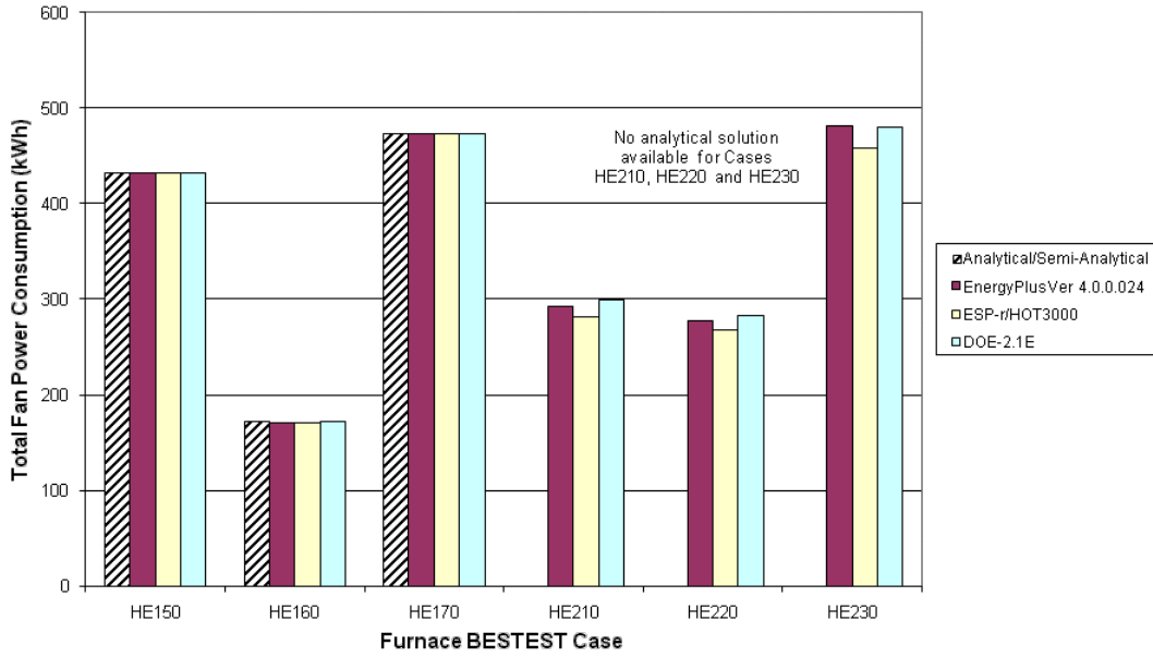
Figure 8 Total Fan Power Results for Various Programs
