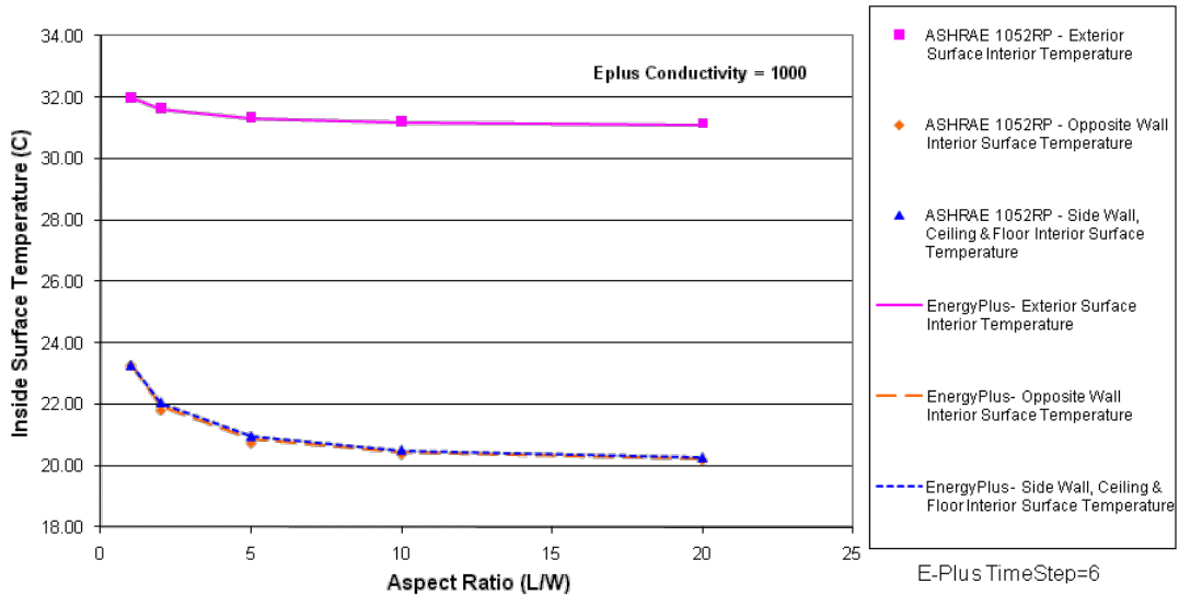
EnergyPlus Version 4.0.0.024 & ASHRAE 1052 Version 1.0 ASHRAE Analytical Test IntRad-Test 3 Exterior Wall Surface Temperature versus Aspect Ratio Building of 3mx3m Cross-Section of Varying Length (L=3xAR) All Surfaces Emis=0.9 Outdoor Temp=40C, Indoor Temp=20C
