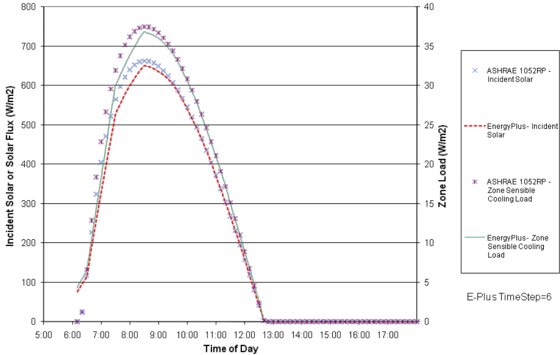
EnergyPlus Version 4.0.0.024 & ASHRAE 1052 ver 1.0 Results for ASHRAE Analytical Test ExtSolRad Atlanta, August 21 East Facing Opaque Surface
