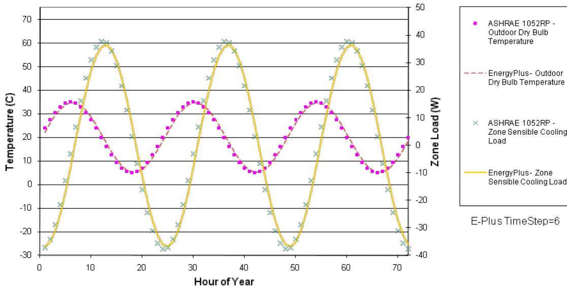
EnergyPlus Version 4.0.0.024 & ASHRAE 1052 Version 1.0 Results for ASHRAE Analytical Test TC3 Transient Conduction, Non-Adiabatic 3-Layer Wall Sinusoidal Change in External Temperature 20C mean, 15C amp, 24 hr period Indoor Temperature Constant at 20C
