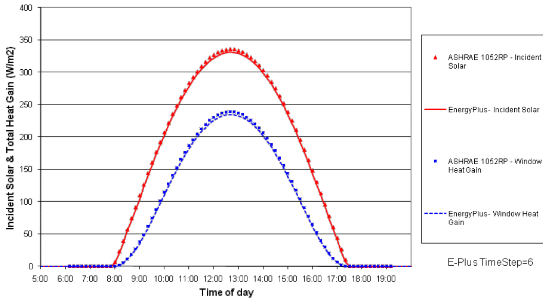
EnergyPlus Version 4.0.0.024 & ASHRAE 1052 Version 1.0 Results for ASHRAE Analytical Test SolRadGlazing Atlanta, August 21 South Facing 1/8" Standard Glass
