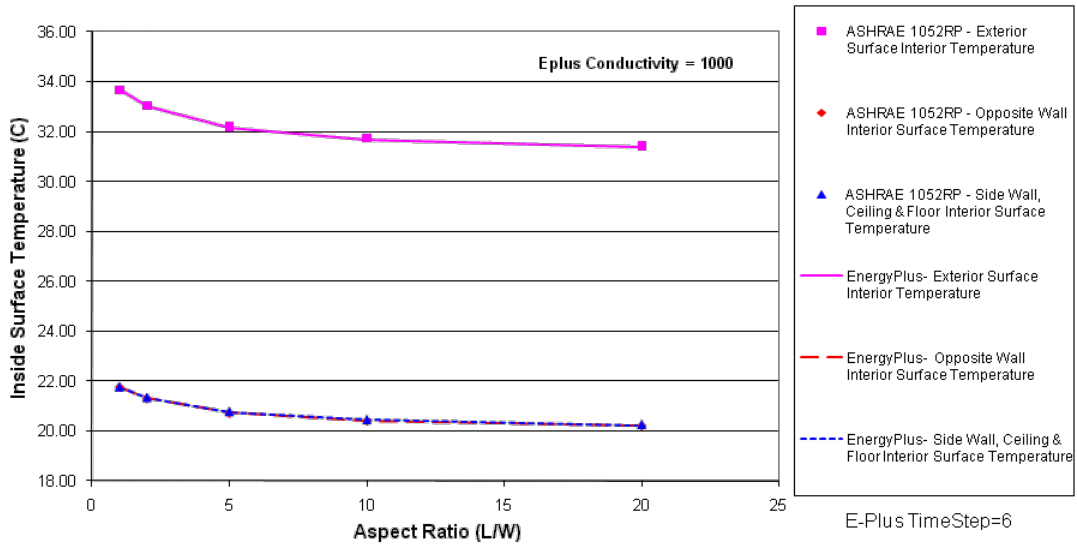
EnergyPlus Version 4.0.0.024 & ASHRAE 1052 Version 1.0 ASHRAE Analytical Test IntLWRad-Test 2 Exterior Wall Surface Temperature versus Aspect Ratio Building of 3mx3m Cross-Section of Varying Length (L=3xAR) Ext. Surface Emis=0.9, All Other Surfaces Emis=0.1 Outdoor Temp=40C, Indoor Temp=20C
