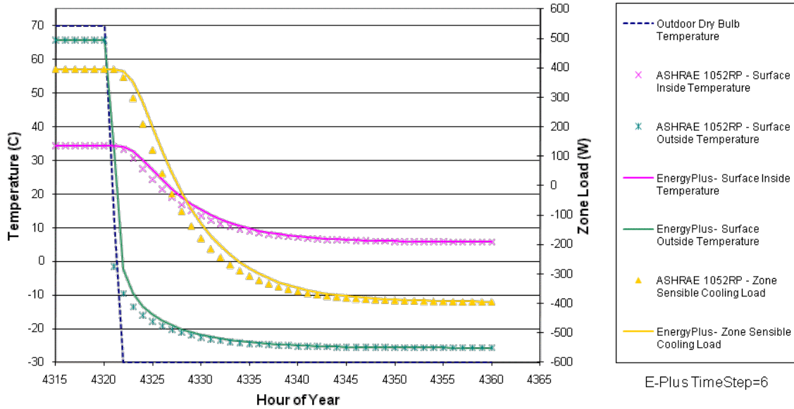
EnergyPlus Version 4.0.0.024 & ASHRAE 1052 Version 1.0 Results for ASHRAE Analytical Test TC2-Step Down Transient Conduction, Non-Adiabatic Wall, 10 cm Wood 100 C Step Change in External Temperature (70C to -30C) Indoor Temperature Constant at 20C
