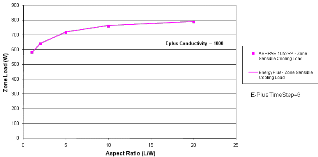
EnergyPlus Version 4.0.0.024 & ASHRAE 1052 Version 1.0 ASHRAE Analytical Test IntLWRad-Test 2 Zone Load versus Aspect Ratio Building of 3mx3m Cross-Section of Varying Length (L=3xAR) Ext. Surface Emis=0.9, All Other Surfaces Emis=0.1 Outdoor Temp=40C, Indoor Temp=20C
