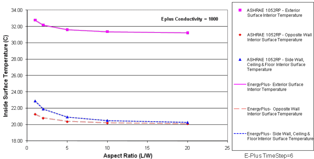
EnergyPlus Version 4.0.0.024 & ASHRAE 1052 Version 1.0 ASHRAE Analytical Test IntLWRad-Test 1 Exterior Wall Surface Temperature versus Aspect Ratio Building of 3mx3m Cross-Section of Varying Length (L=3xAR) Ext. Surf. Emis.=0.9, Oppos. Surf. Emis.=0.1, Other Surf. Emis.=0.3 Outdoor Temp=40C, Indoor Temp=20C
