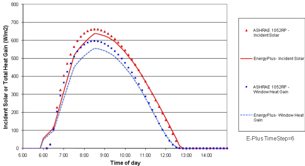
EnergyPlus Version 4.0.0.024 & ASHRAE 1052 Version 1.0 Results for ASHRAE Analytical Test SolRadGlazing Chicago, August 21 East Facing 1/8" Standard Glass
