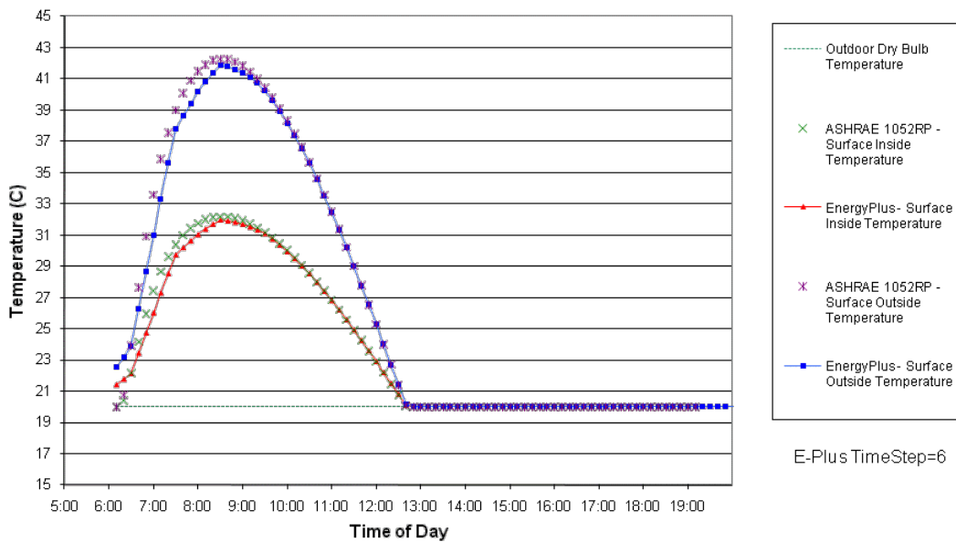
EnergyPlus Version 4.0.0.024 & ASHRAE 1052 ver 1.0 Results for ASHRAE Analytical Test ExtSolRad Atlanta, August 21 East Facing Opaque Surface
